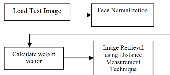
Fig. 2: Processing of test image and retrieval flowchart
